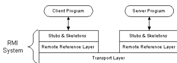
Figure 7. RMI Layered Structure
