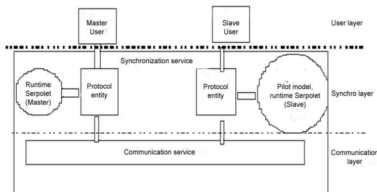
Figure 1. Copy synchronization protocol architecture.
