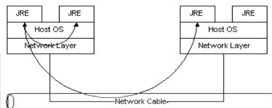
Figure 8. Transport Layer
